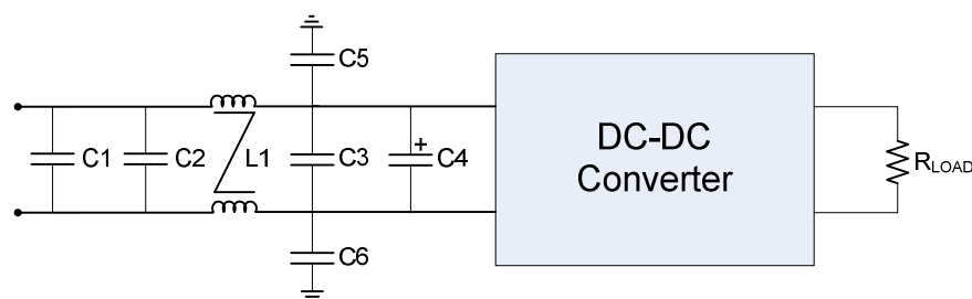
Figure 15. EMI Filter
