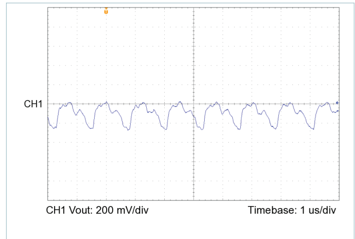
Figure 18 — Output voltage ripple, V_{IN} = 43\text{V} , V_{OUT} = 12.0\text{V} , C_{OUT\_EXT} = 1000\mu\text{F} , R_{LOAD} = 1.429\Omega
