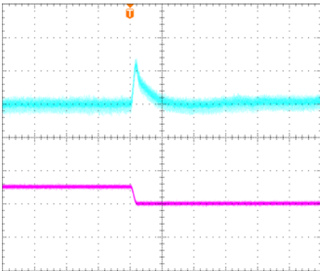
Figure 7: Transient Response (V_{in}=48V, 1A/\mu s\ step\ change\ in\ load\ from\ 50\% \ to\ 75\% \ of\ I_{o,max}) V_{out} (top trace): 100mV/div, 100us/div; I_{out} (bottom trace): 25A/div. Scope measurement should be made using a BNC cable (length shorter than 20 inches). Position the load between 51 mm to 76 mm (2 inches to 3 inches) from the module 820uF Oscon, 33uF*6 MLCC, 1uF Ceramic, 10uF Tantalum.
