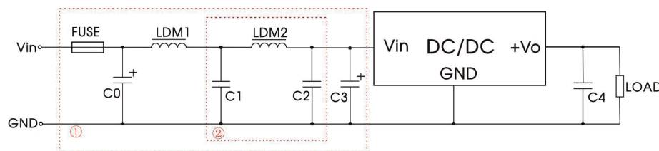
Fig.4 Recommended compliance circuit
