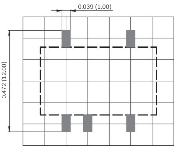
PCB Printing Layout
