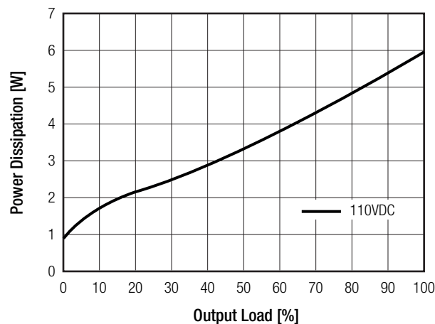
Dissipation vs. Load
