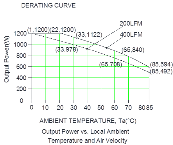
Figure 25. For 0RQP-X5M12B
