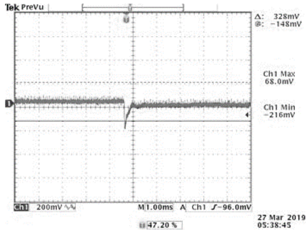
Figure 13. 50%-75% Load Transients at V_{in} = 54\text{ V} @ T_a = 25^\circ\text{C}
