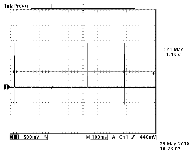
Figure 21. Over current protection V_{in} = 54\text{V} @ T_a = 25^\circ\text{C} ; CH1: Output Voltage
