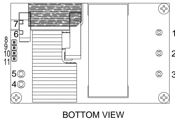
Figure 35. Pins
