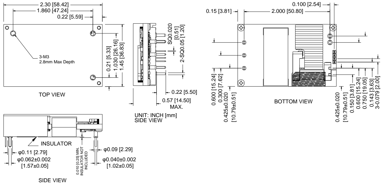
Figure 32. 0RQP-X5M12AG outline
