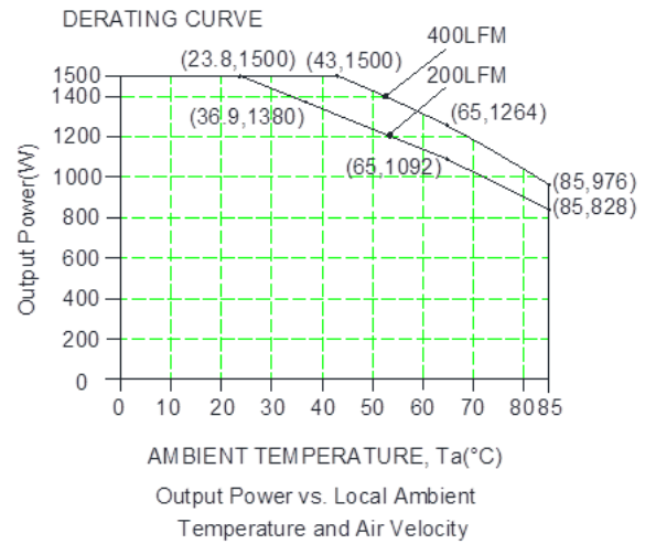
Figure 26. For 0RQP-X5M12B + External heatsink
