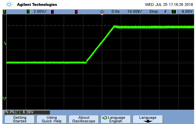
Figure 25 Output Pre-bias start-up Vin=48V, Iout = 0A, Cload = 10000 \mu F, Ta = 25°C, Pre-bias Voltage = 9.6V
