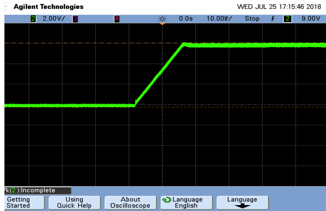
Figure 24. Output Pre-bias start-up Vin=48V, Iout = 0A, Cload = 47 \mu F, Ta = 25°C, Pre-bias Voltage = 9.6V
