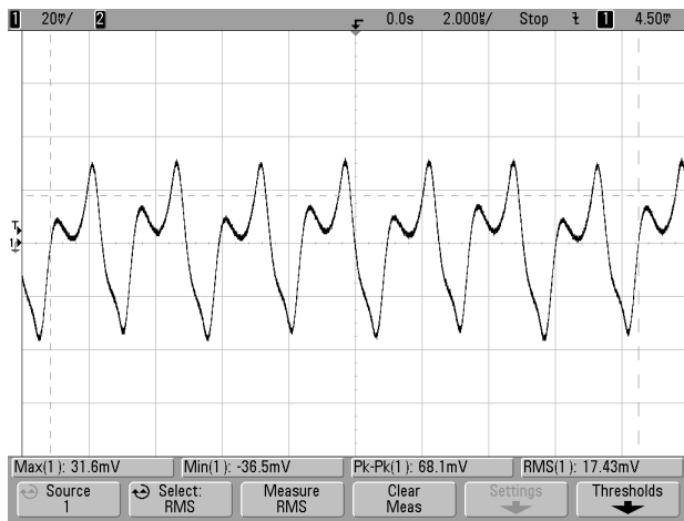
Figure 16. Ripple/Noise @+25°C (Vin=48V, Iout=0A, Cload=330μF, Scope BW=20MHz, 2μS/div, 20mV/div)
