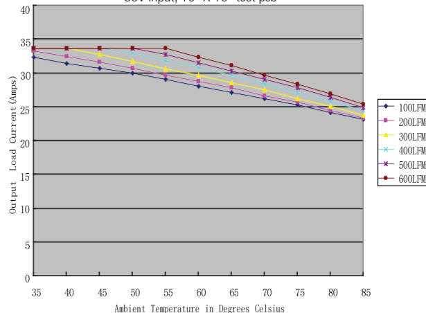
Figure 13. Temperature derating, current, longitudinal airflow Vin to Vout 48V Input, 10" X 10" test pcb
