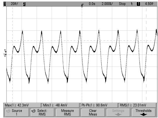
Figure 17. Ripple/Noise @+25°C (Vin=48V, Iout=33A, Cload=330μF, Scope BW=20MHz, 2μS/div, 20mV/div)
