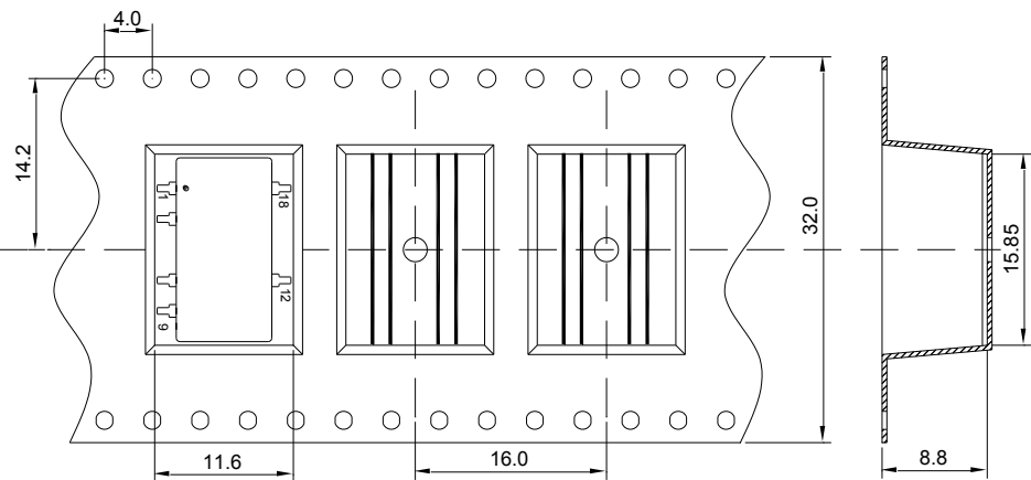
Tape & Reel
