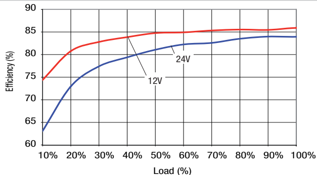
NCS6D4805C
