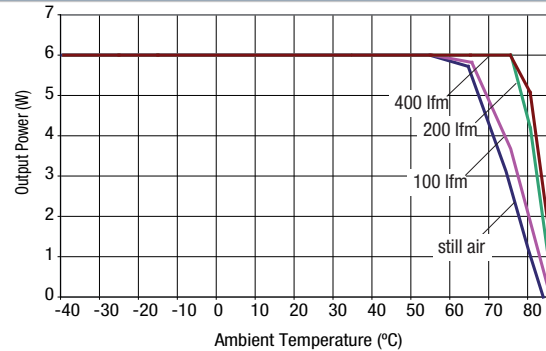
NCS6D4815C
