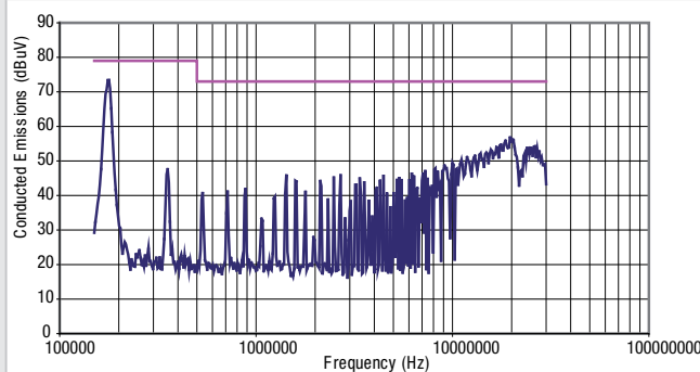
NCS6S4815C
