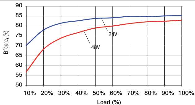
NCS6D4812C
