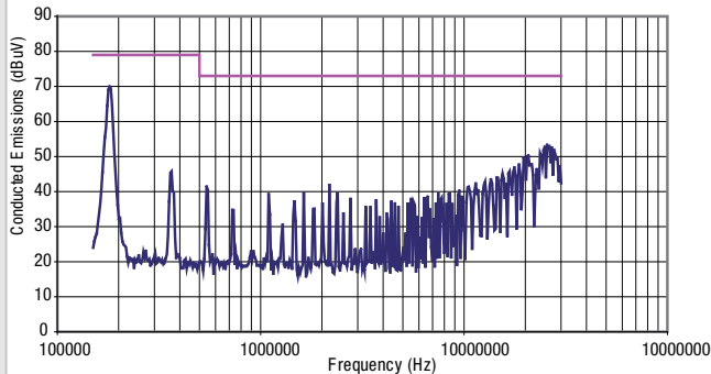
NCS6S4805C
