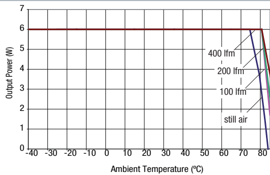
NCS6D1215C
