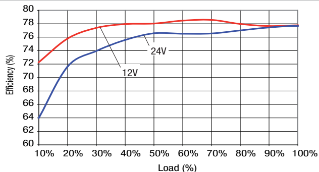
NCS6D1215C
