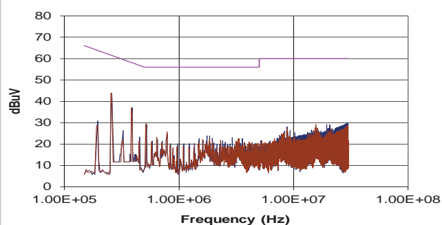
NMK0505TSAC (Quasi-Peak)
