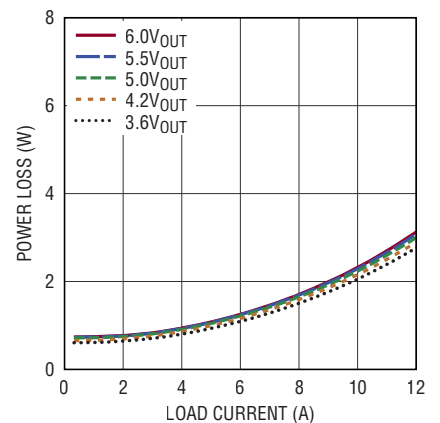
Power Loss vs Load, 12V_{IN} , f_{SW} = 800\text{kHz}
