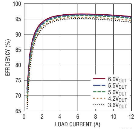
Efficiency vs Load, 12V_{IN} , f_{SW} = 800\text{kHz}
