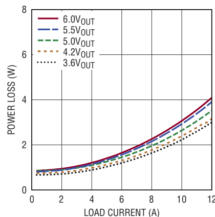
Power Loss vs Load, 12V_{IN} , f_{SW} = 600\text{kHz}
