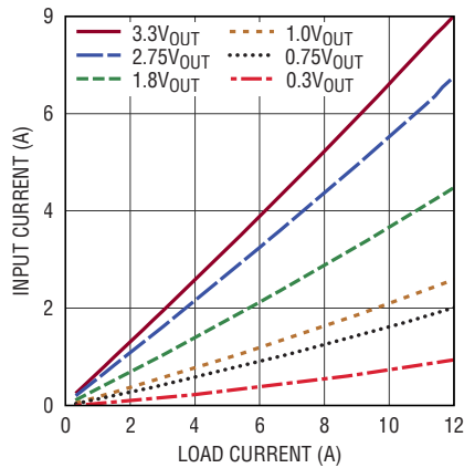
Input vs Load, 5\text{V}_{\text{IN}} , f_{\text{SW}} = 400\text{kHz}
