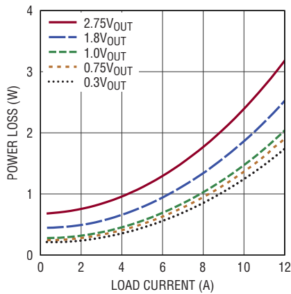
Power Loss vs Load, 12V_{IN} , f_{SW} = 400\text{kHz}
