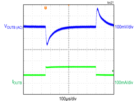
MAXM17715-MAXM17720, MAXM17721-MAXM17726 LOAD TRANSIENT RESPONSE
