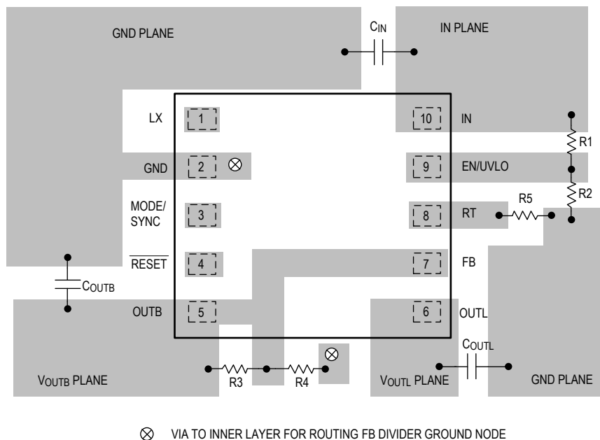
Figure 4. Adjustable Output Layout Guidelines
