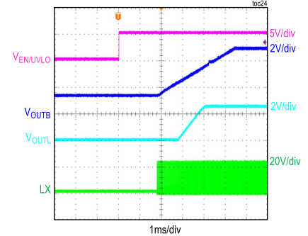
MAXM17724 STARTUP THROUGH ENABLE (1.5V PREBIAS)
