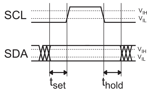
Setup and hold times timing diagram
