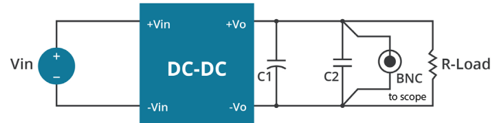
Figure 2 Measuring Output Ripple And Noise
