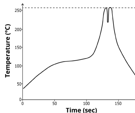
WAVE SOLDERING PROFILE
