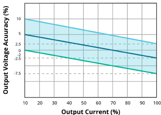
OUTPUT REGULATION CURVE 5 Vdc input model / 5, 9, 12, 15, 24 Vdc output models (nominal input)
