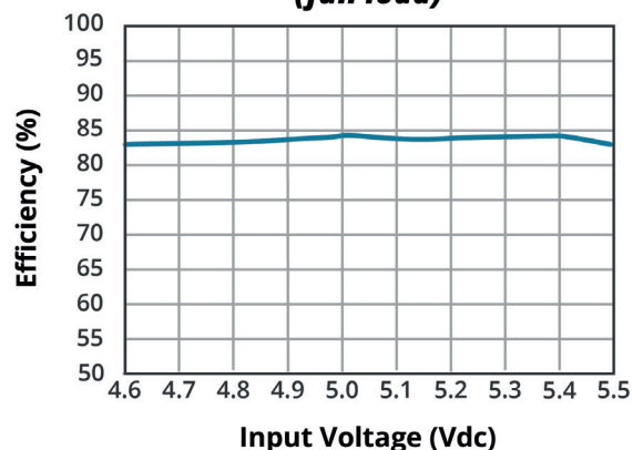
EFFICIENCY VS INPUT VOLTAGE PDSE2-S5-S5-M (full load)
