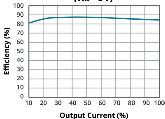
EFFICIENCY VS OUTPUT LOAD PDSE2-S5-S5-M (Vin = 5 V)
