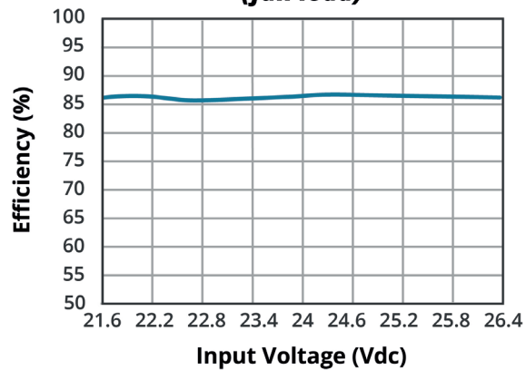
EFFICIENCY VS INPUT VOLTAGE PDSE2-S24-S5-M (full load)
