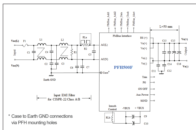
PFH500A Basic Connection Diagram
