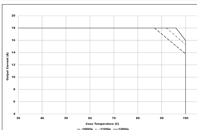
PFH500A-28 Derating Curve
