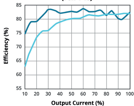
EFFICIENCY VS OUTPUT LOAD (PSK-4-15)
