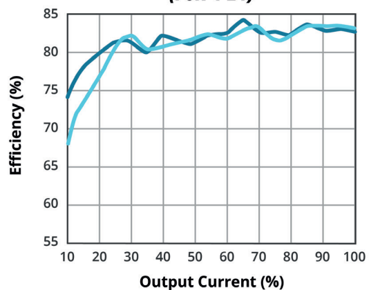
EFFICIENCY VS OUTPUT LOAD (PSK-4-24)
