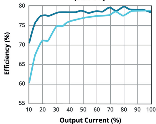
EFFICIENCY VS OUTPUT LOAD (PSK-4-5)
