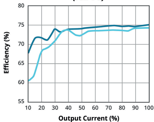
EFFICIENCY VS OUTPUT LOAD (PSK-4-3)
