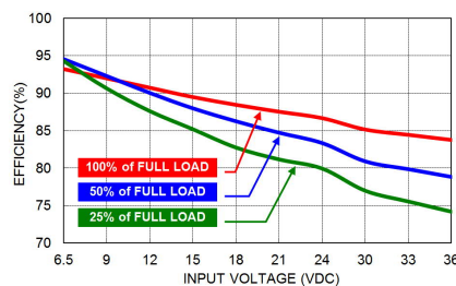
PSR1.0-5P0 Efficiency vs. Input Voltage
