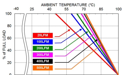
PSR1.0-5P0 Derating Curve High VIN
