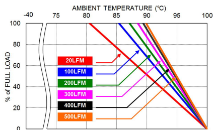
PSR1.0-5P0 Derating Curve LOW VIN
