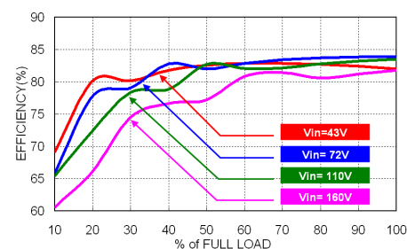
RDL06-110S05W Efficiency vs. Output Load
