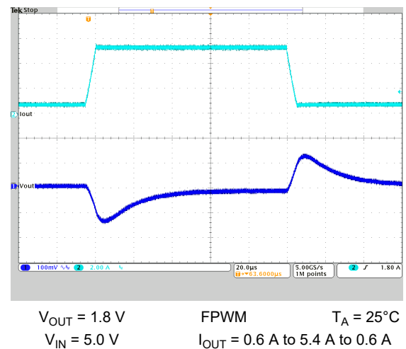
Figure 8-25. Load Transient Response
