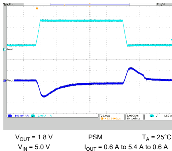
Figure 8-24. Load Transient Response
