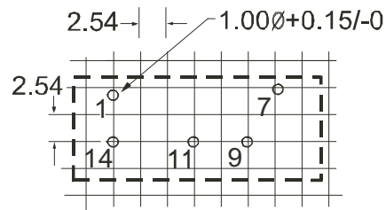
Layout
