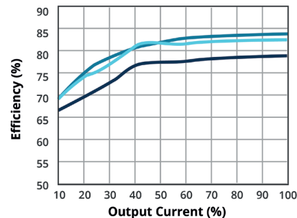
EFFICIENCY VS OUTPUT LOAD (at 230 Vac)
