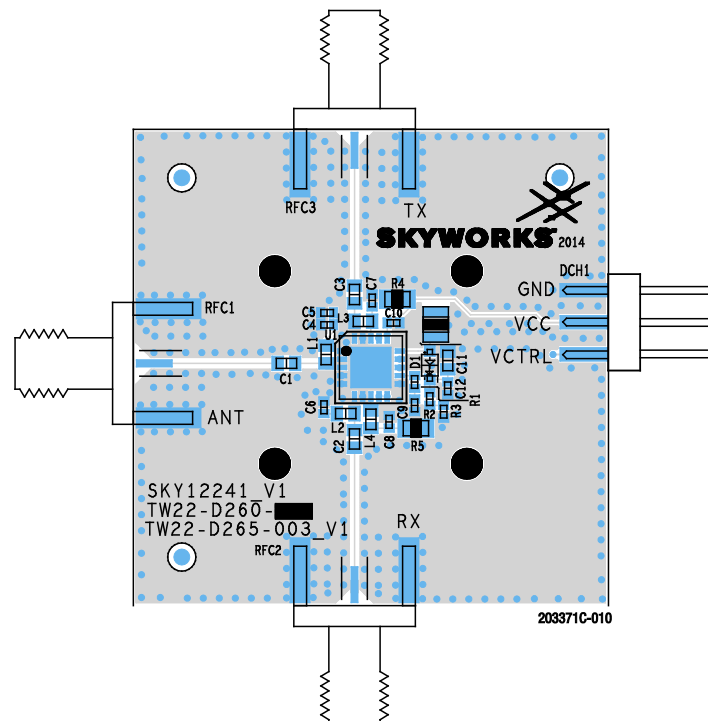
Figure 10. SKY12241-492LF Evaluation Board Assembly Diagram
