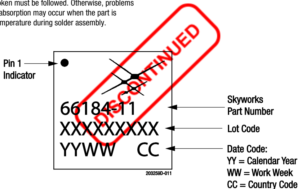
Figure 11. Typical Part Marking
