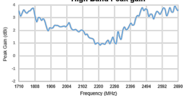
High Band Peak gain
