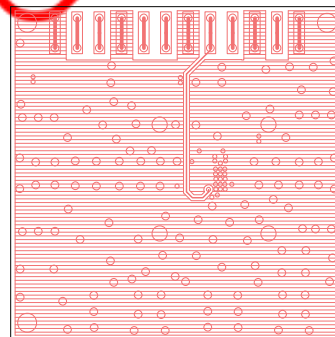
Layer 3: Ground
