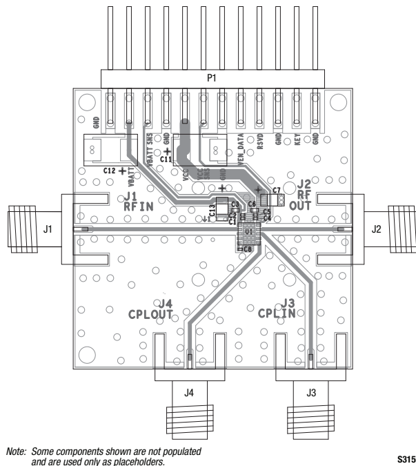
Figure 11. SKY66002-11 Evaluation Board Assembly Diagram
