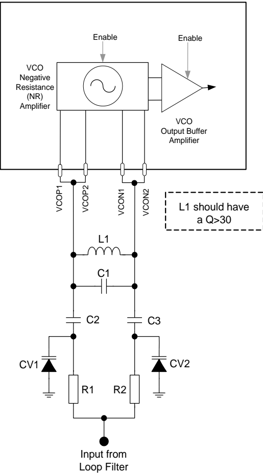
Figure 11 Example External Components – VCO External Tank Circuit
