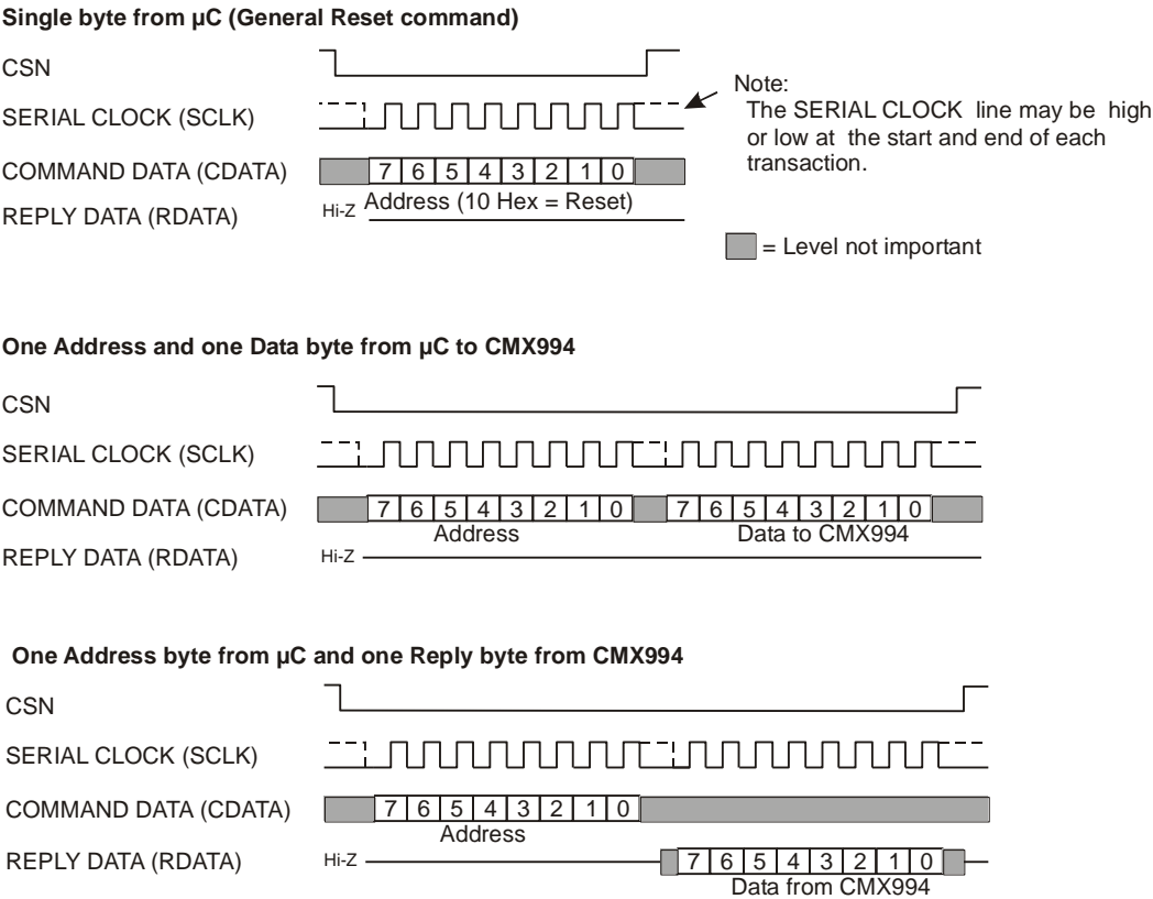
Figure 17 C-BUS Transactions
