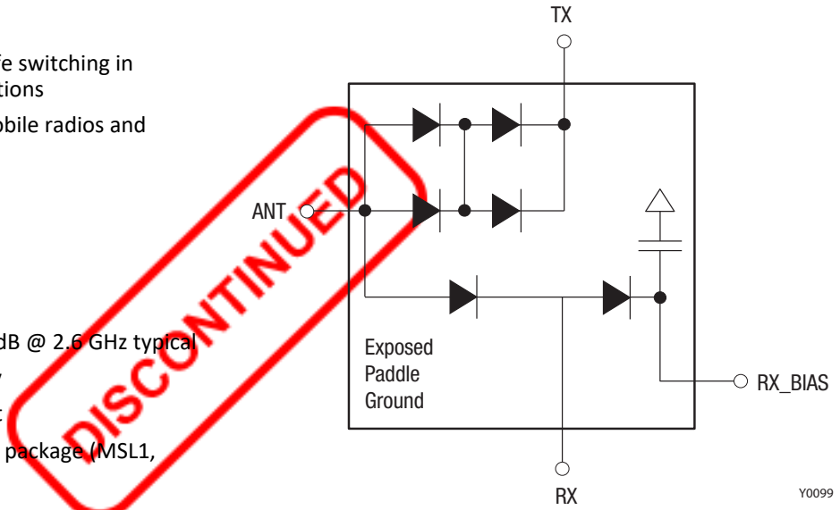
Figure 1. SKY12215-478LF Block Diagram
