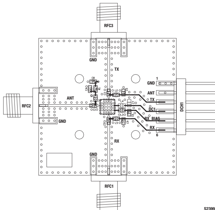
Figure 10. SKY12215-478LF Evaluation Board Assembly Diagram
