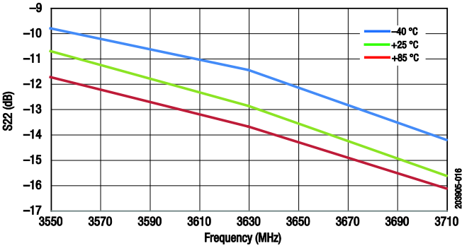
Figure 16. Output Return Loss vs Frequency Across Temperature (Small Signal, PIN = -20 dBm)
