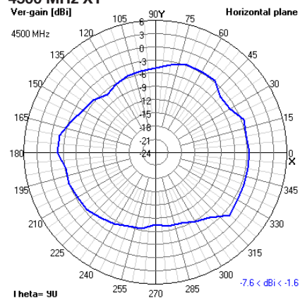
4500 MHz XY
