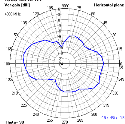
4000 MHz XY
