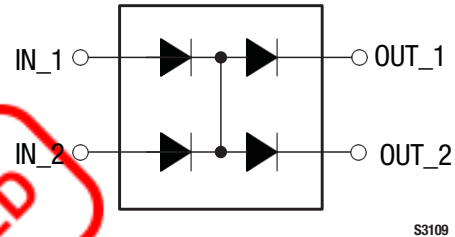
Figure 1. SKY12213-478LF Block Diagram
