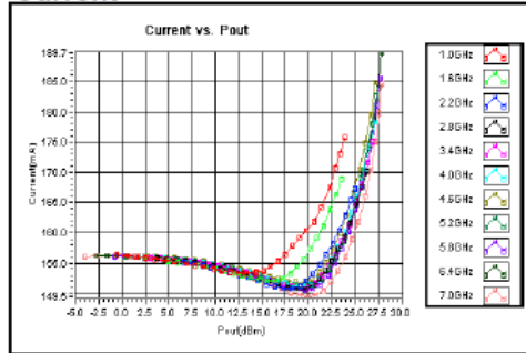
Current
