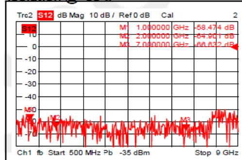
Isolation @+85°C
