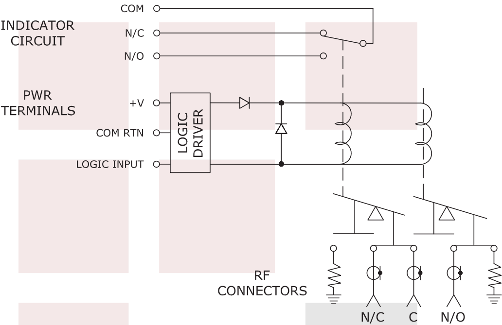
SCHEMATIC FAILSAFE IN NORMALLY CLOSED POSITION
