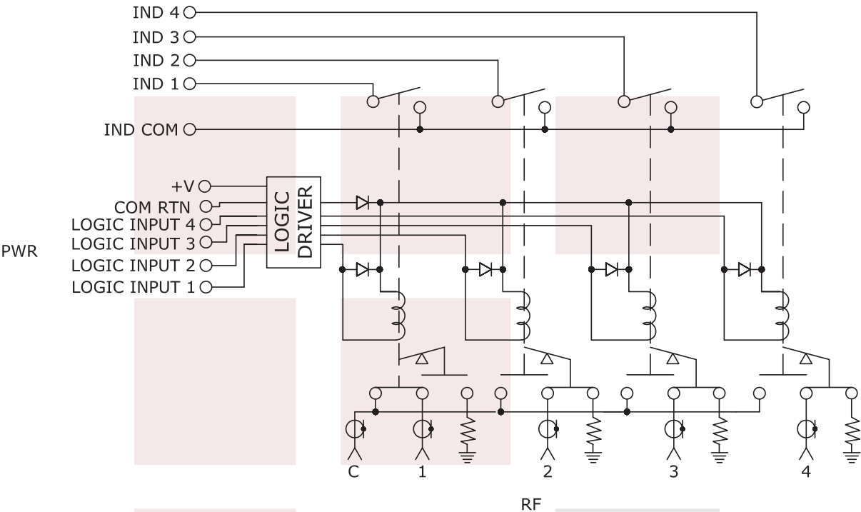
SCHEMATIC NORMALLY OPEN SHOWN IN DE-ENERGIZED POSITION
