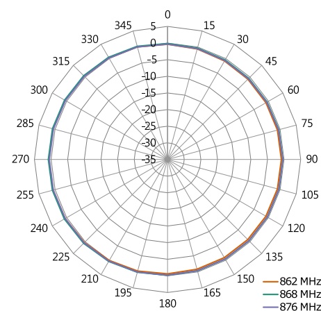
XY-Plane Gain
