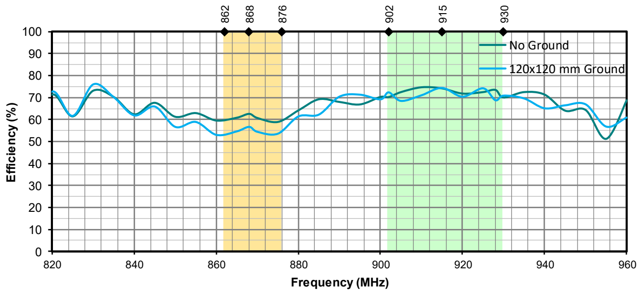
Figure 8. Antenna Efficiency
