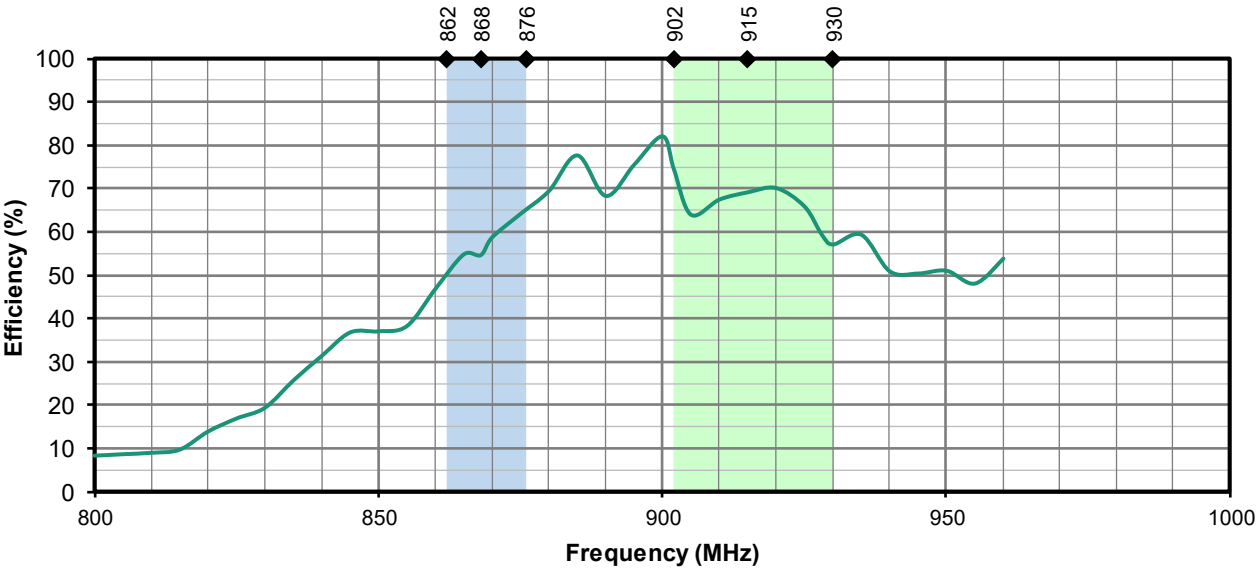
Figure 8. Antenna Efficiency
