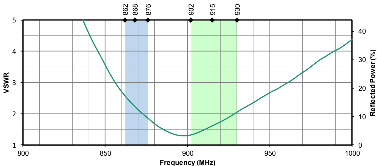
Figure 4. Antenna VSWR
