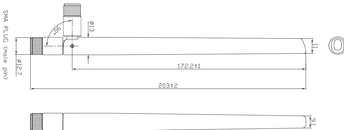
Figure 2. Antenna Dimensions
