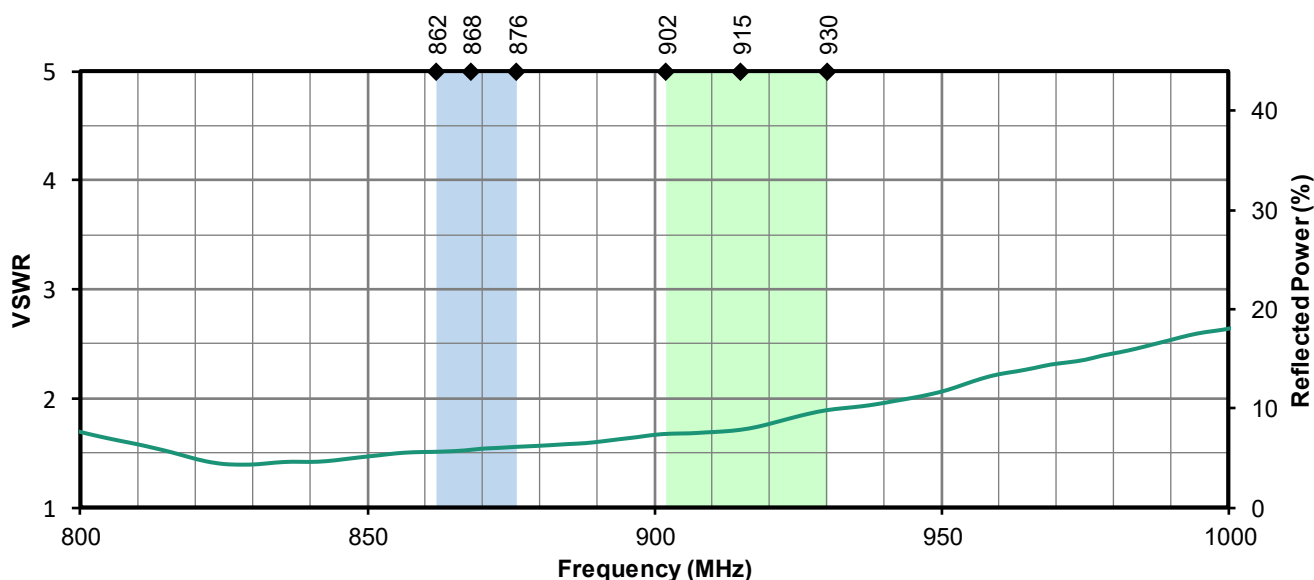
Figure 4. Antenna VSWR, Edge Bent 90 Degrees
