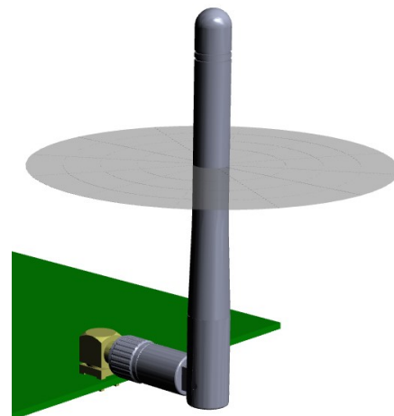
XY-Plane Gain
