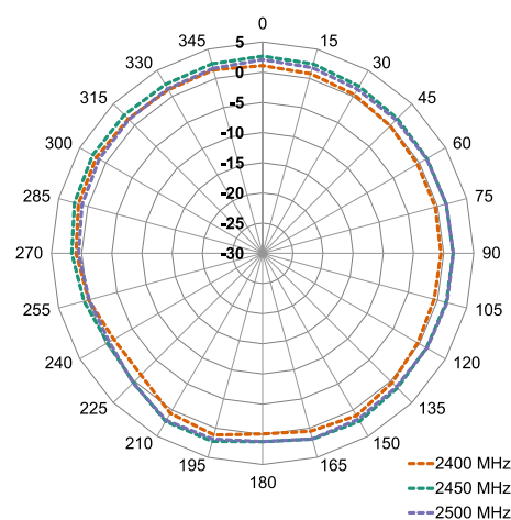
XY-Plane Gain
