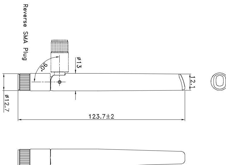
Figure 2. Antenna Dimensions
