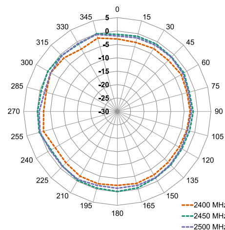
XY-Plane Gain
