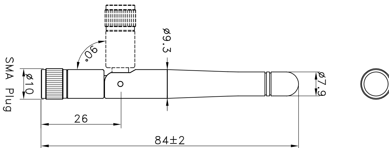
Figure 2. Antenna Dimensions
