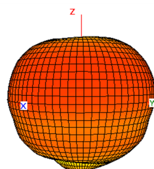
2500 MHz
