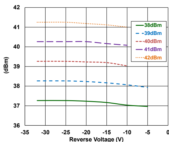
Output Power over Reverse Bias Voltage @ +85°C, 29 GHz
