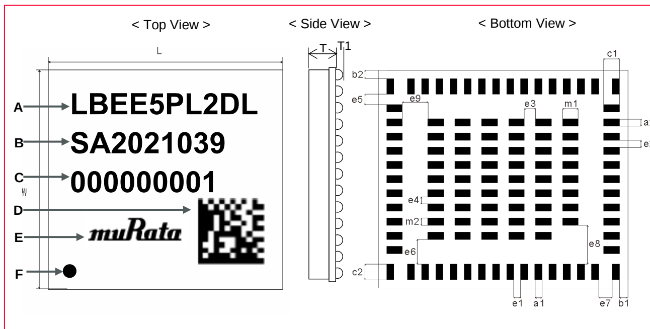
Figure 3: Dimensions and Terminal Configurations Markings
