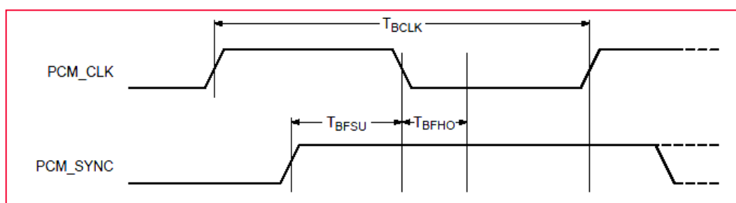
Figure 21: PCM_SYNC Signals (Slave Mode)
