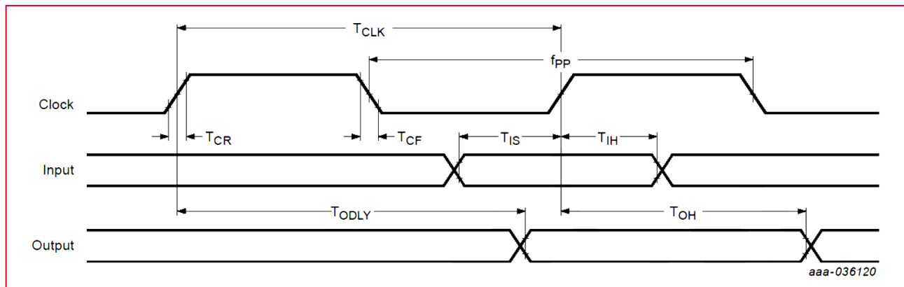
Figure 13: SDR12, SDR25, and SDR50 modes at 1.8V (up to 100 MHz)
