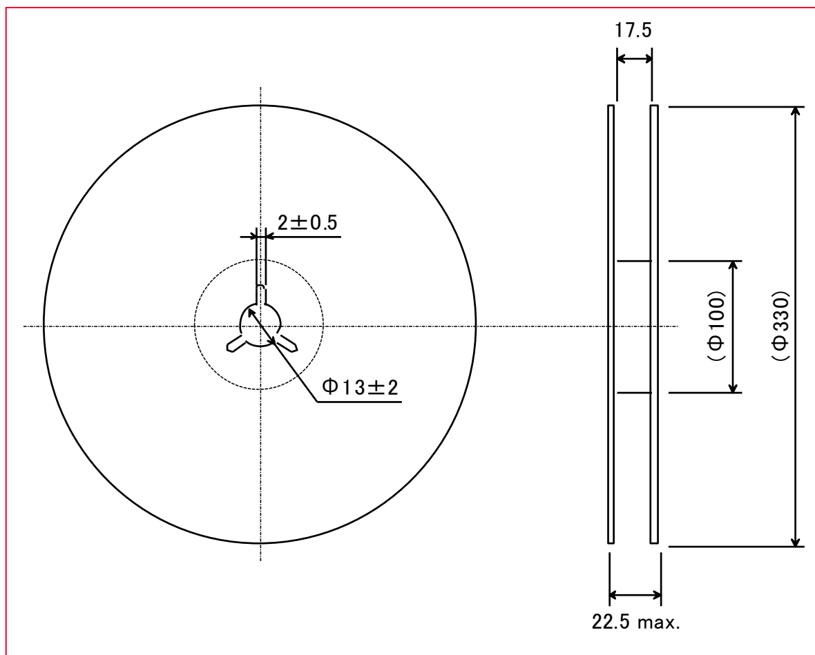
Figure 25: Dimensions of Reel (Unit: mm)
