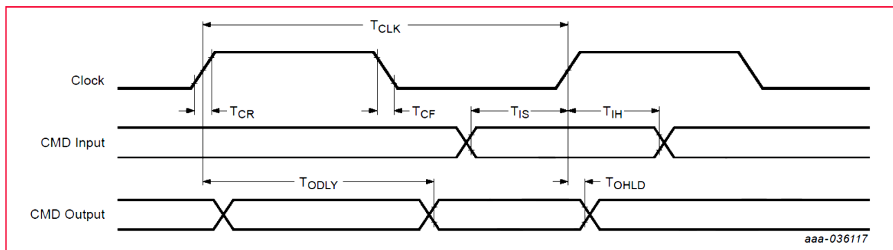
Figure 15: DDR50 Mode at 1.8V (50 MHz)
