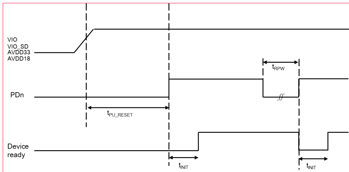
Figure 10: Hot Reset Sequence
