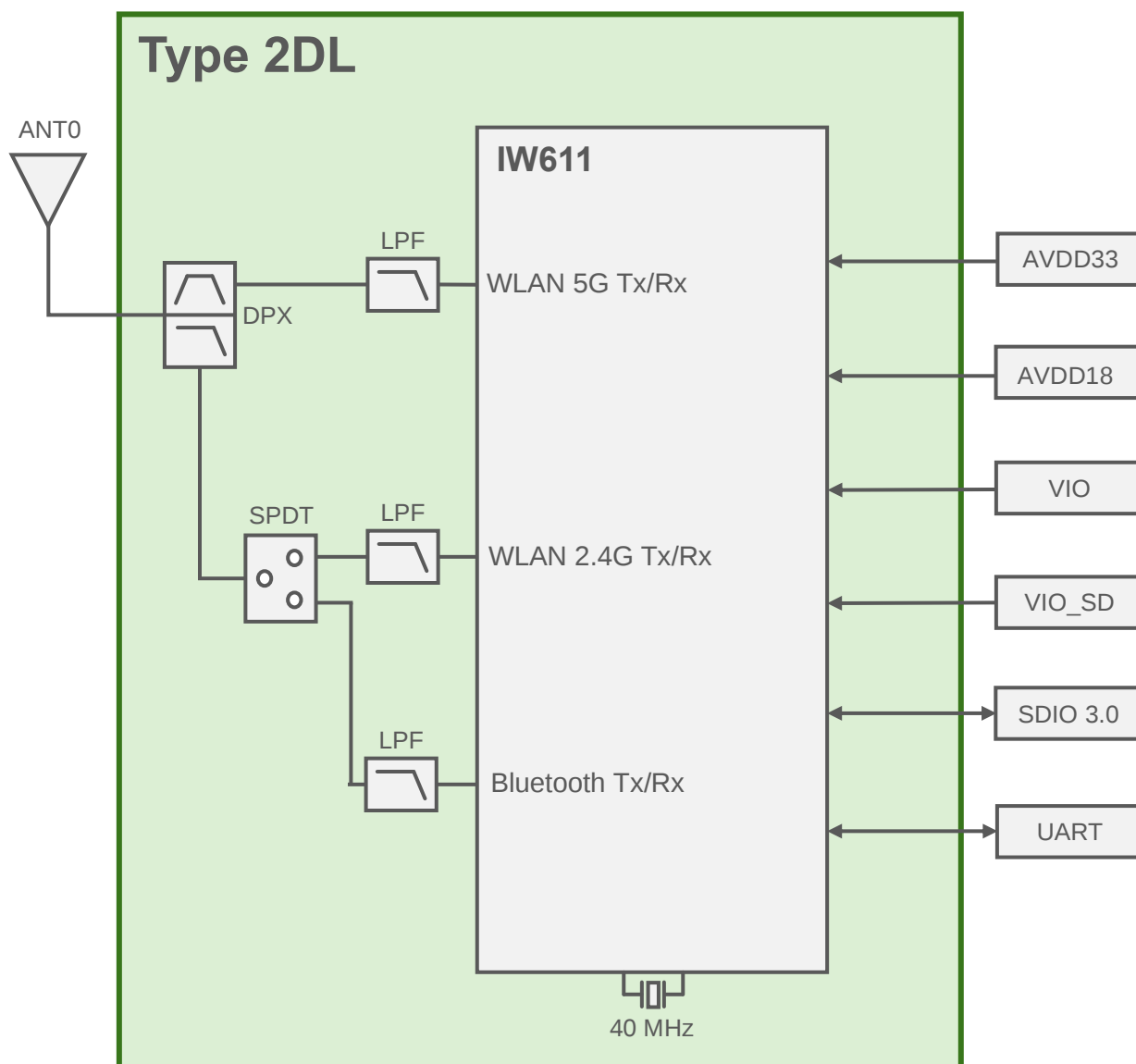
Figure 1: Block Diagram - Type 2DL for the shared WLAN-Bluetooth antenna
