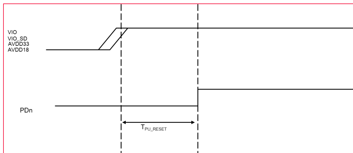
Figure 8: Power-On Sequence
