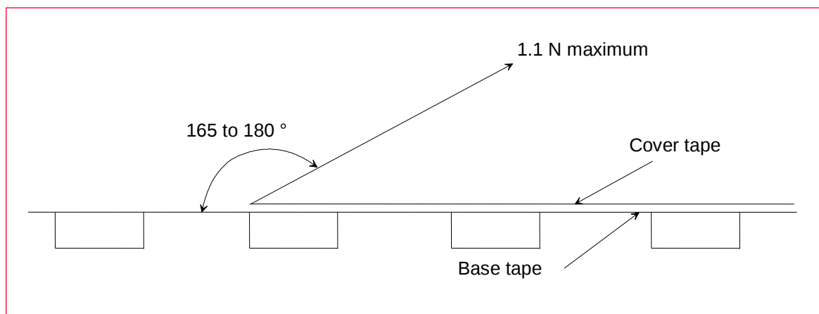
Figure 28: Peeling Force
