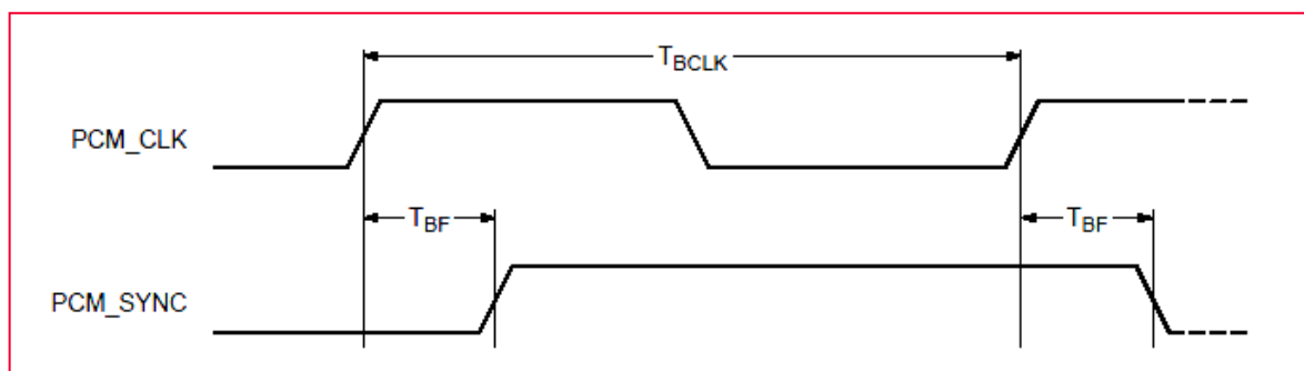
Figure 19: PCM_SYNC Signals (Master Mode)
