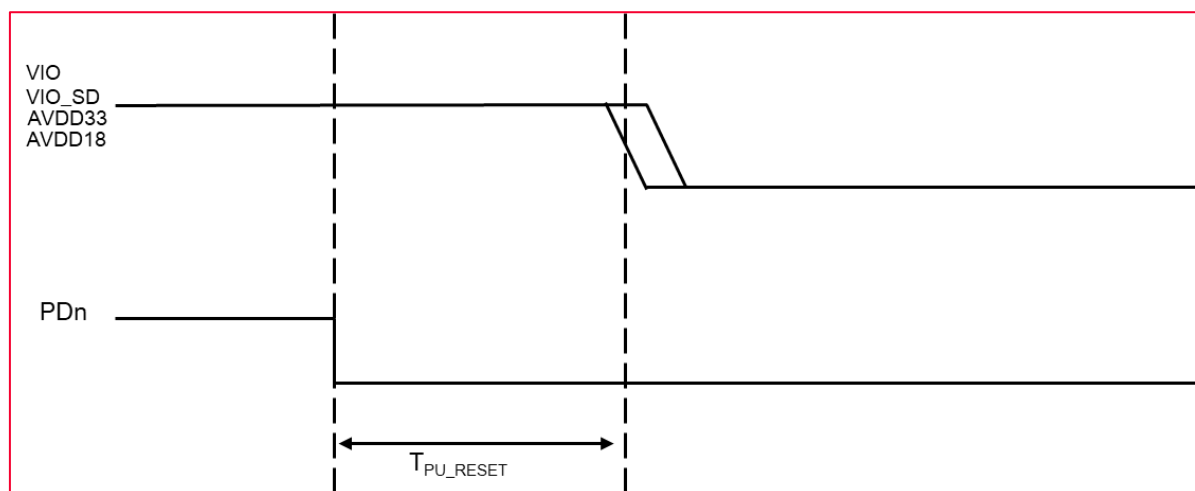
Figure 9: Power-Off Sequence
