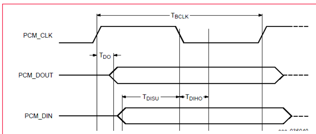
Figure 20: Data Signals (Slave Mode)
