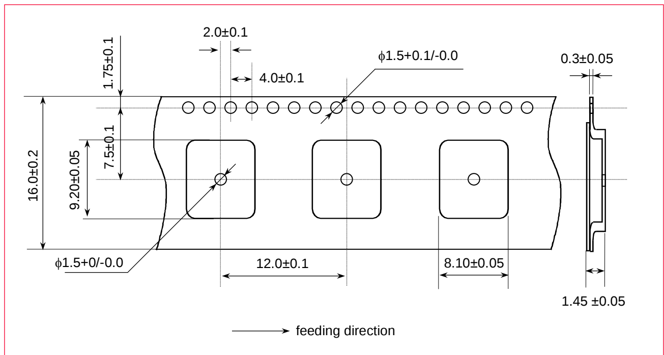
Figure 24: Dimensions of Tape (Plastic Tape)
