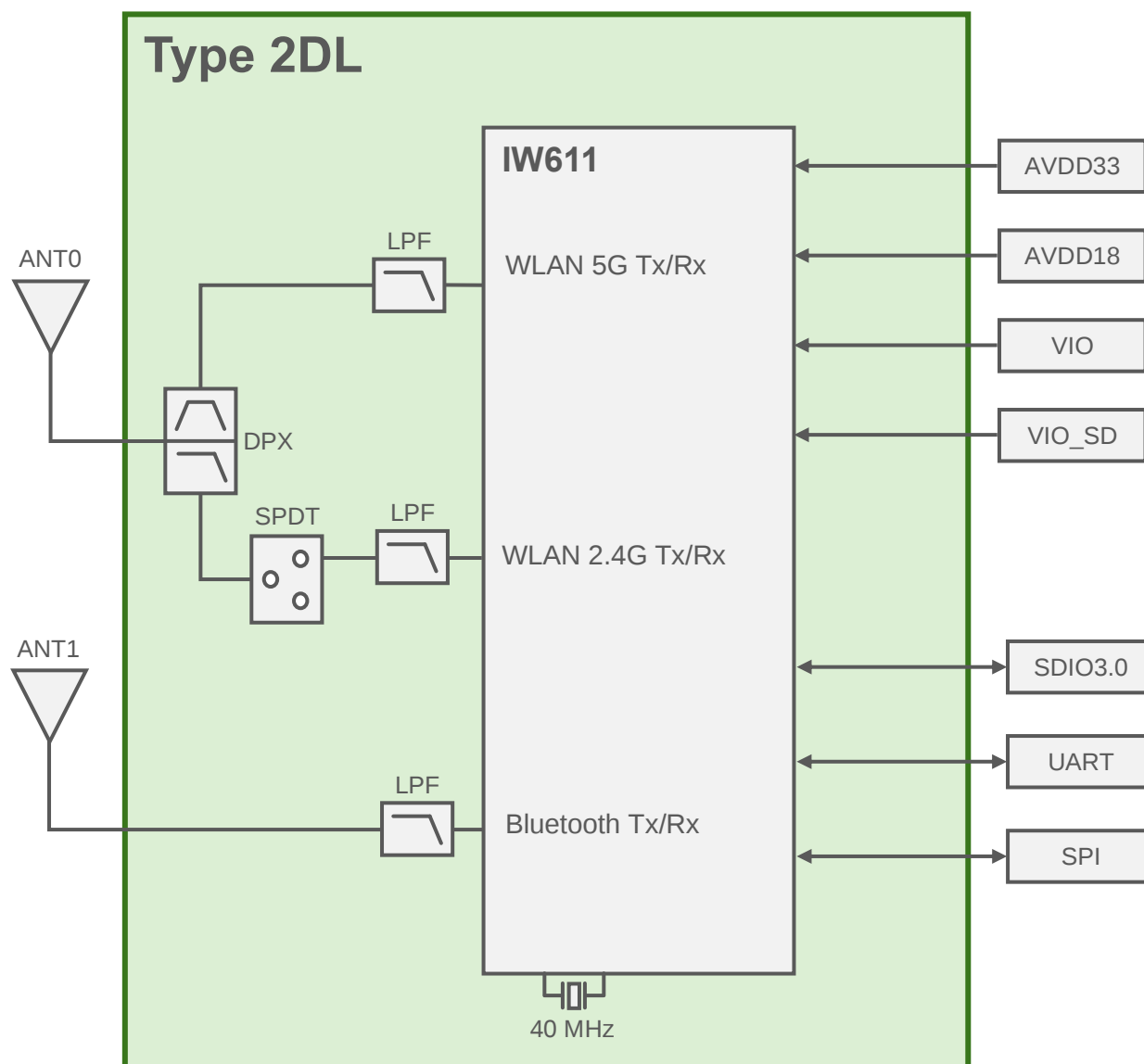
Figure 2: Block Diagram - Type 2DL for the dedicated Bluetooth antenna
