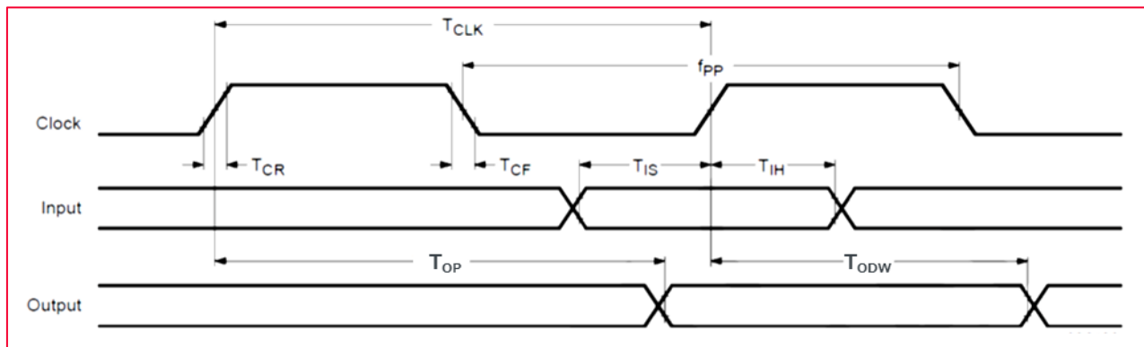
Figure 14: SDR104 mode at 1.8V (208 MHz)
