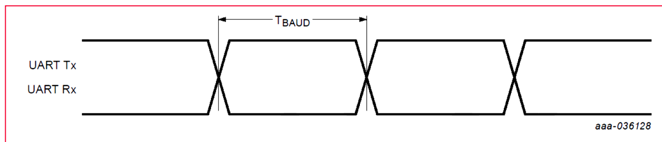
Figure 17: UART Timing Default Mode Signals
