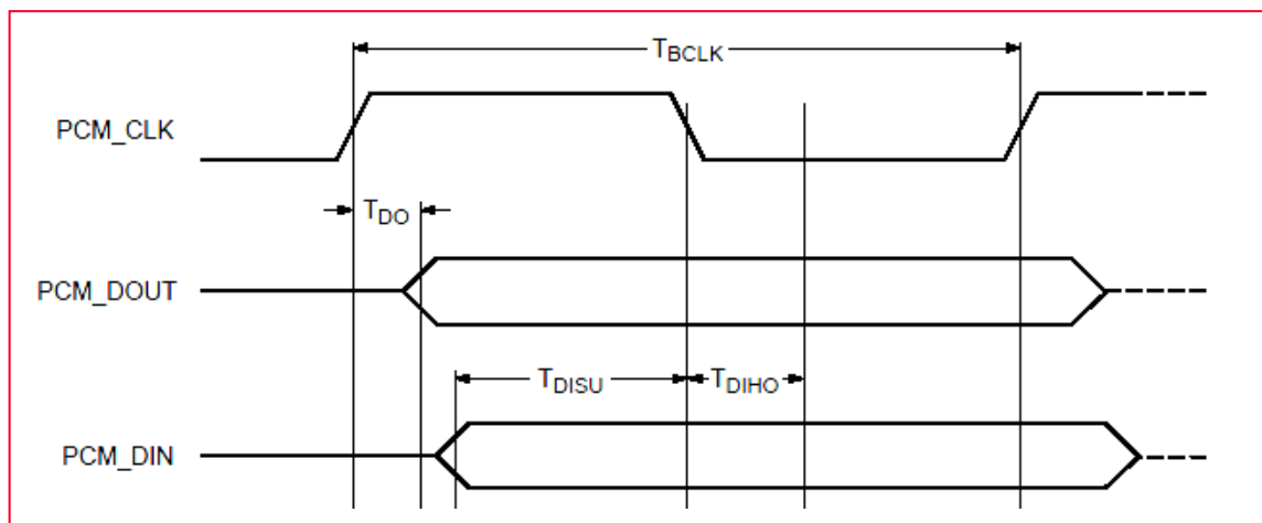
Figure 18: Data Signals (Master Mode)
