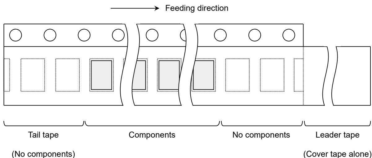
Figure 16: Leader and Tail Tape
