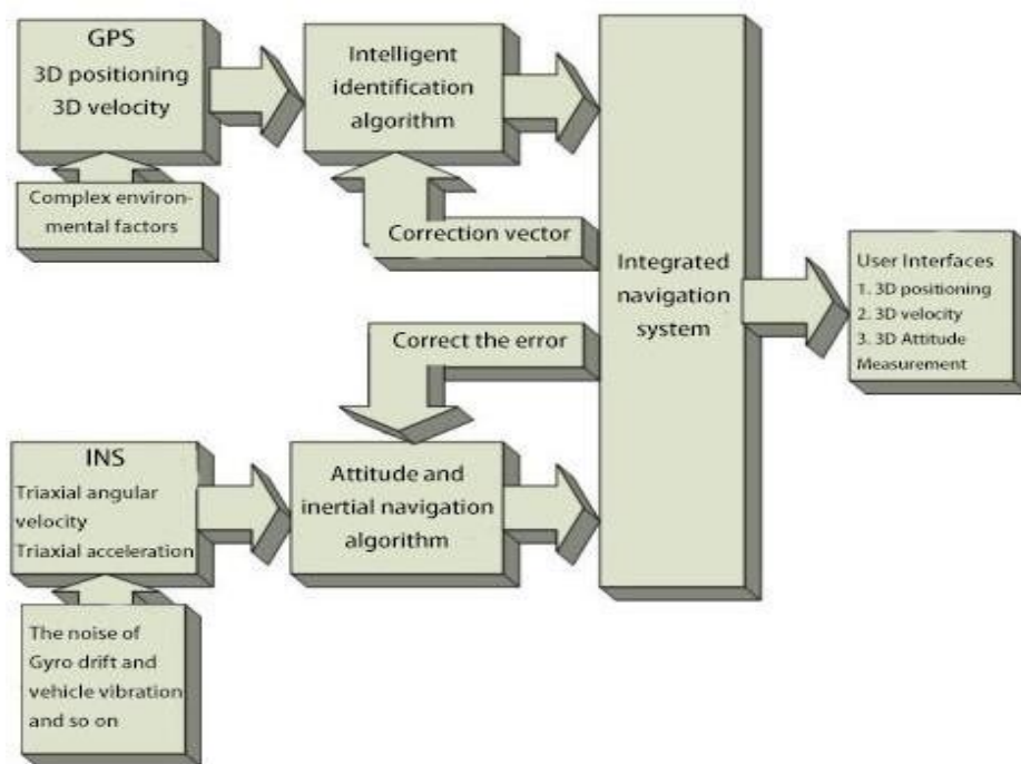
Figure 1-2 : Block Diagram
