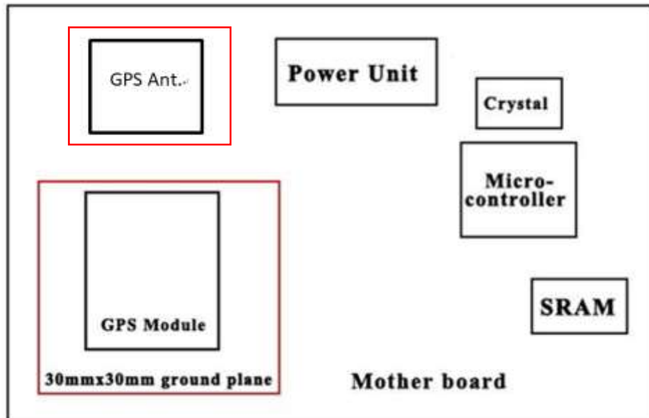
Figure 9: Recommended Placement of GNSS Antenna and Module
