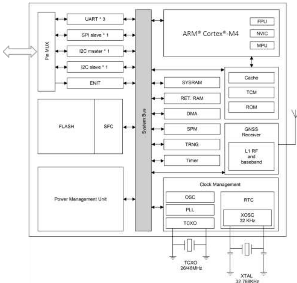
Figure 1: Block Diagram
