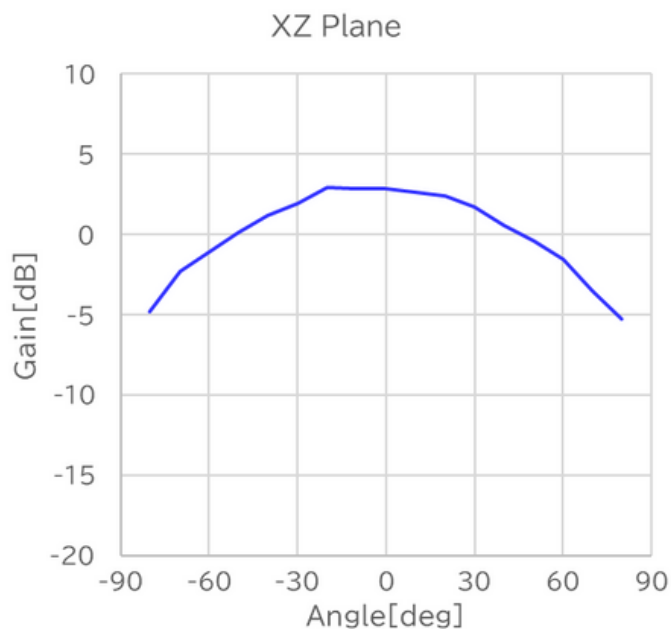
Radiation Pattern 1207.14MHz
