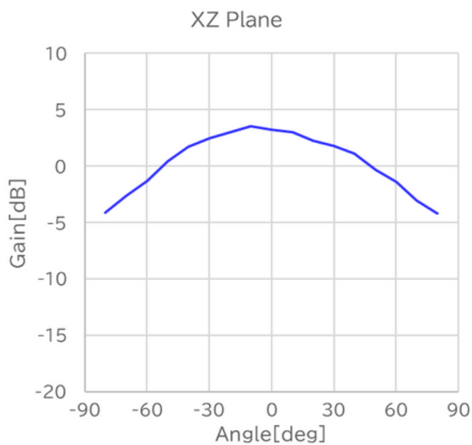
Radiation Pattern 1227.6MHz
