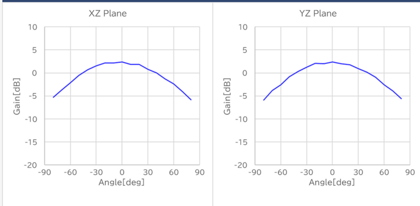
Radiation Pattern 1245.78MHz
