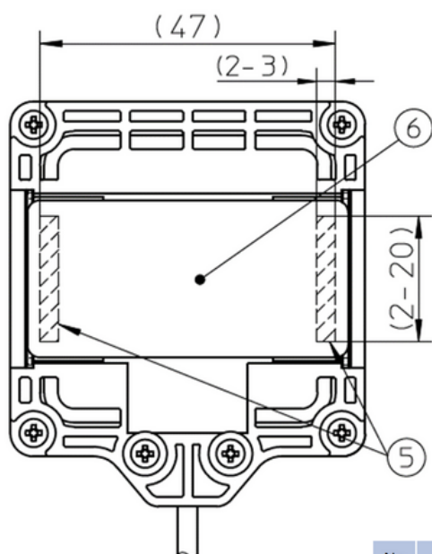
BOTTOM VIEW
