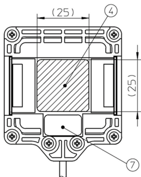
BOTTOM VIEW
