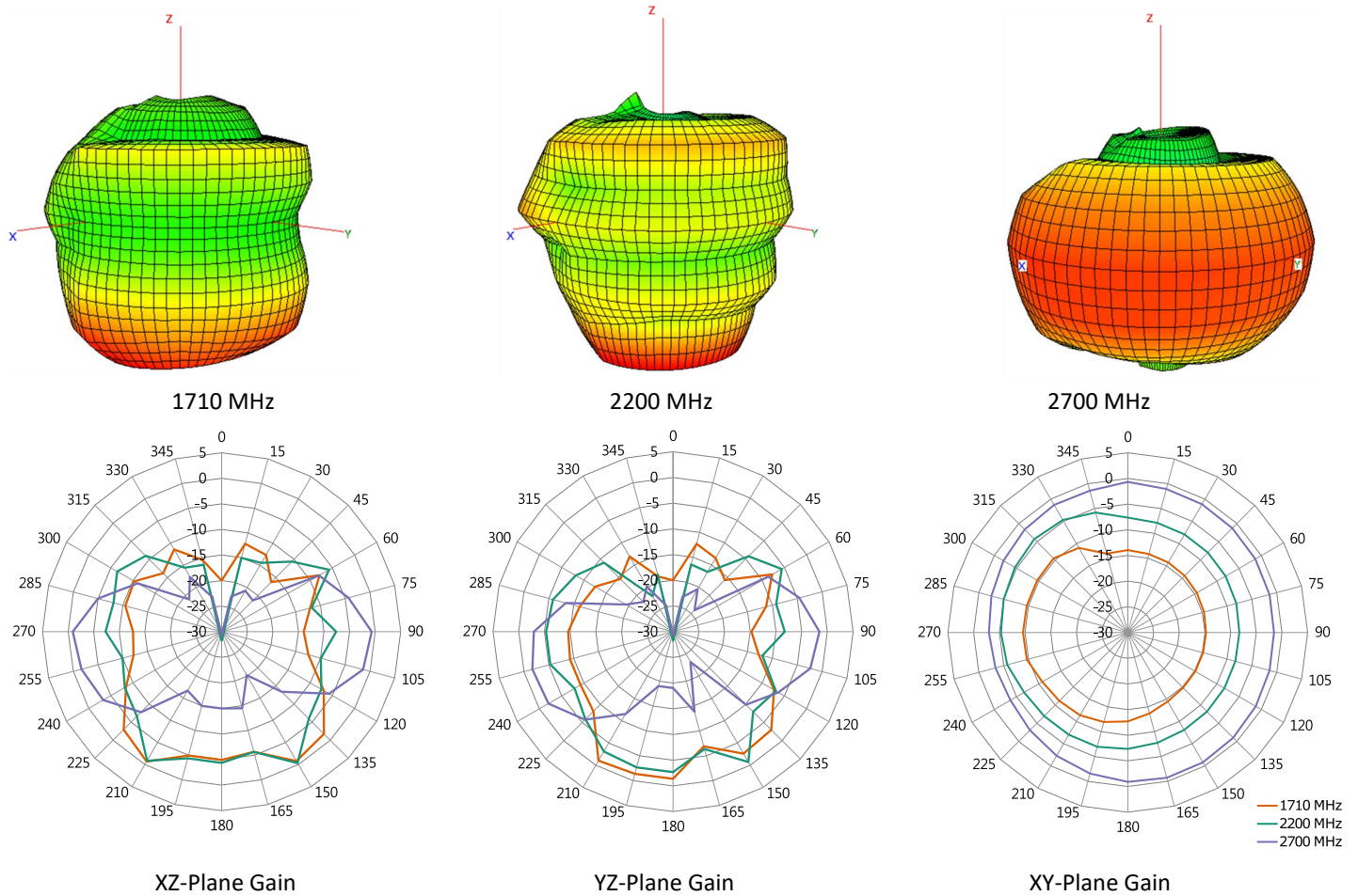
Figure 10-1. Antenna Radiation Patterns, Straight without ground plane
