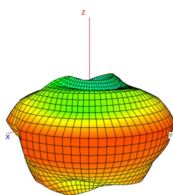
617 MHz
