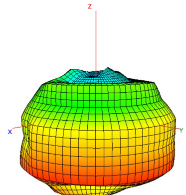
960 MHz
