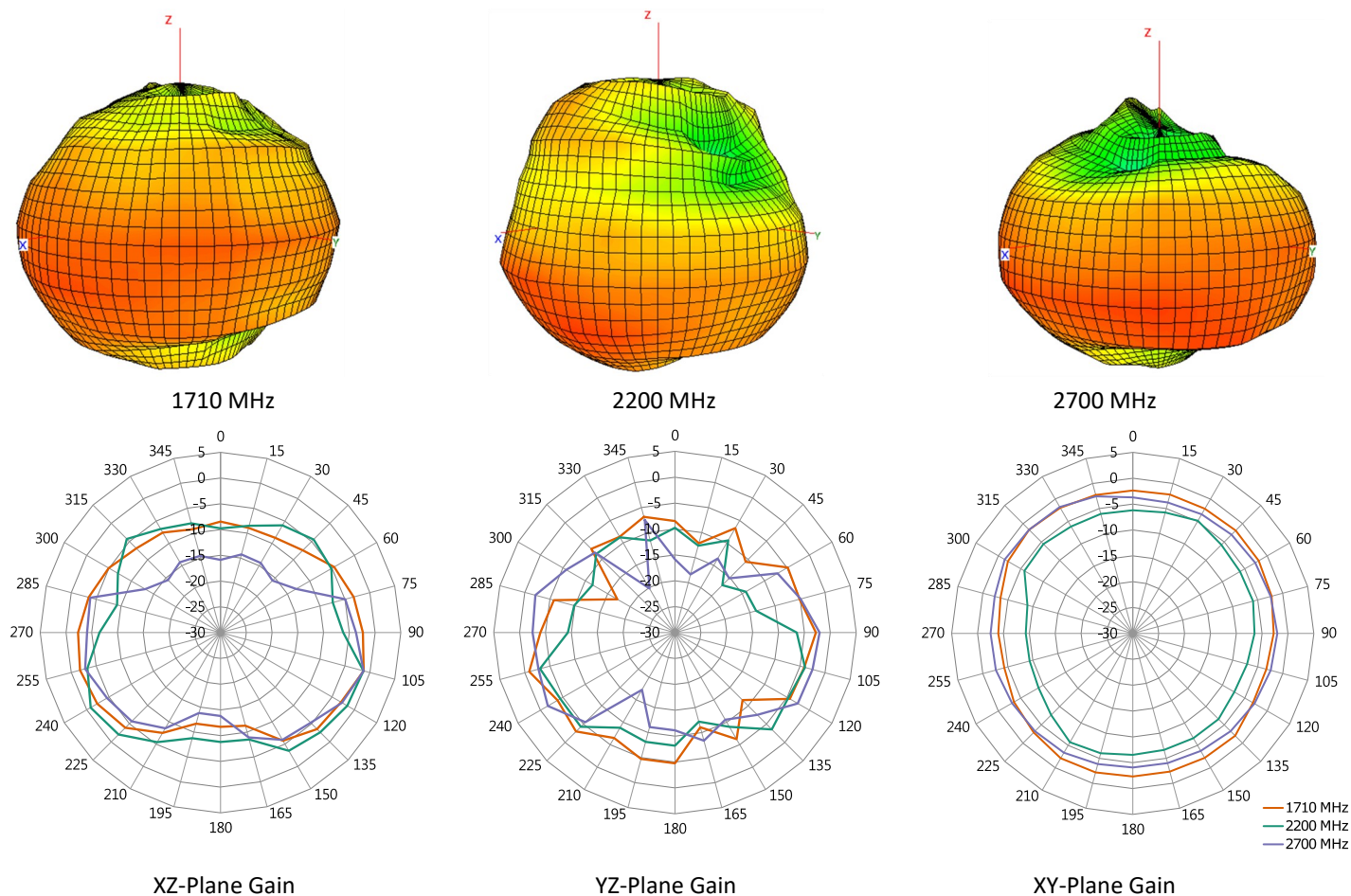
Figure 17-1. Antenna Radiation Patterns, Edge Bent 90 Degrees
