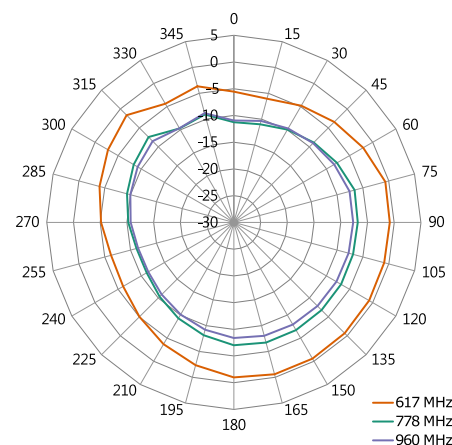
XY-Plane Gain
