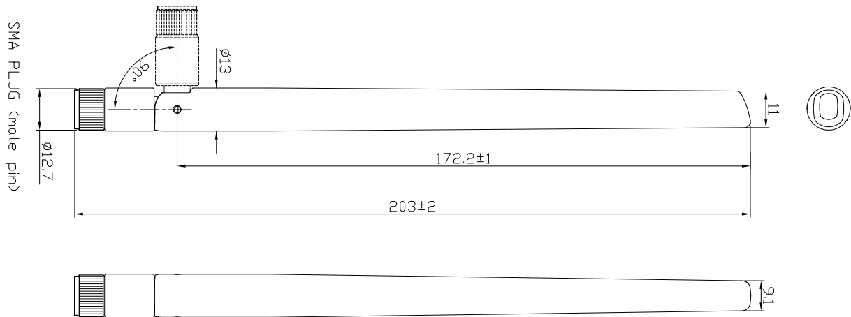
Figure 2. Antenna Dimensions
